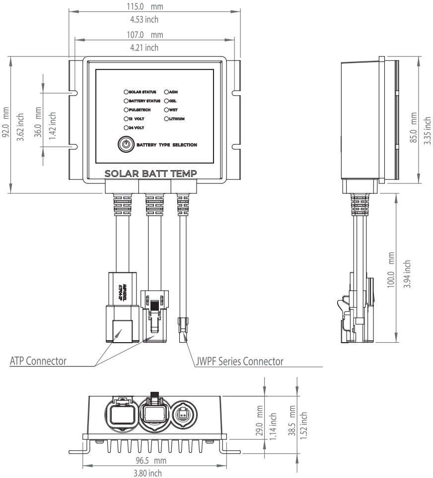
Figure 4: PT20 Mounting Diagram
